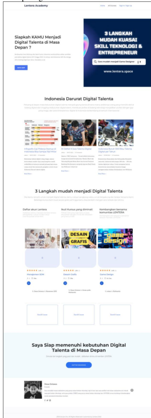
Gambar 2. Dashboard Lentera
